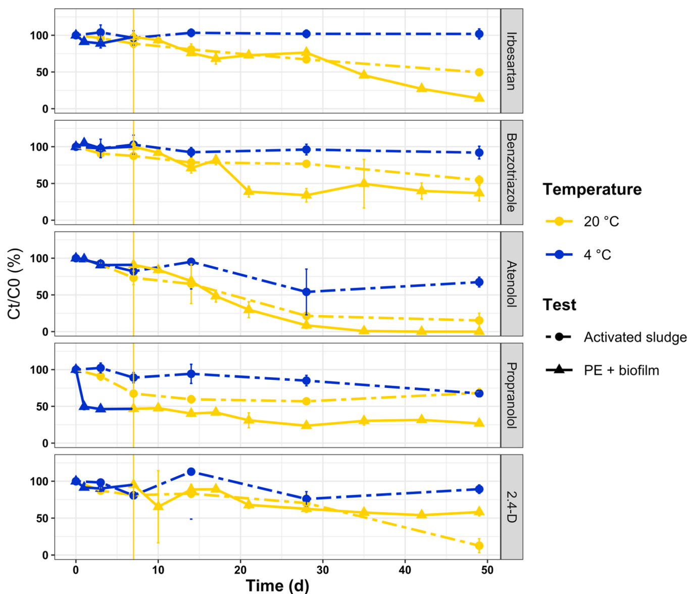
Fig. 4. Fraction (%) of irbesartan, benzotriazole, atenolol, propranolol, and 2,4-D remaining in batches over time (d). Lines and points represent the average of three replicates. Starting concentration was 1 µg/L, other concentration can be found in the supplementary materials A (Fig. S4) . Error bars represent the standard deviation between the replicates. The vertical yellow line (7d) represents the temperature change from 4 °C (blue solid line, ▲) to 20 °C (yellow solid line, ▲) for the batches with PE + biofilm.
