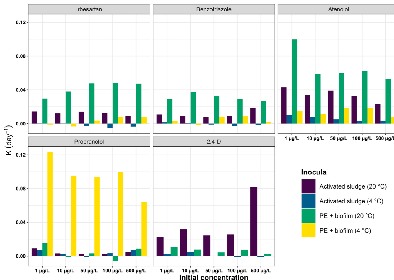
Fig. 5. Removal rate ( k ) ( \text{day}^{-1} ) for irbesartan, benzotriazole, atenolol, propranolol and 2,4-D as a function of initial concentration level. K was extracted from the pseudo-first-order kinetic models (Eq. 5). Batches with PE + biofilm were incubated at 4 °C for 7 d and then at 20 °C for 42 d.
