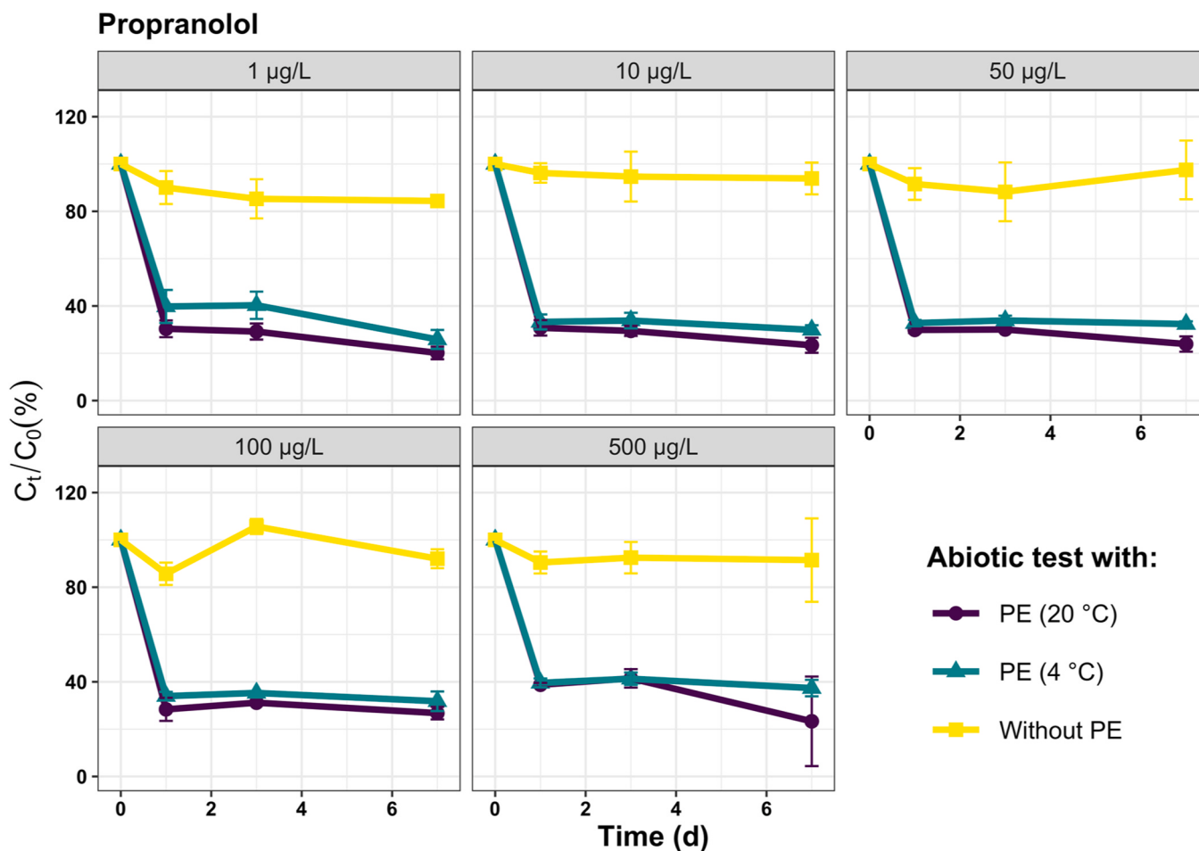
Fig. 2. Fraction of propranolol (%) remaining in abiotic removal tests. Points and lines represent the average ( n=3 ) of each test over time (d). Error bars represent the standard deviation between the triplicate.
