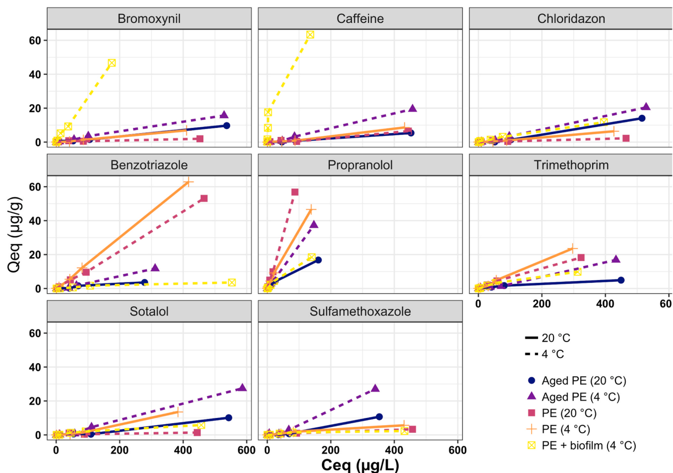
Fig. 3. Isotherm sorption analysis of eight selected OMPs. Dashed and full lines represent the experimental temperature (dashed= 4 °C, full= 20 °C). Colors and dot shape represent each individual experiment. PE + biofilm (4 °C) data were extracted from the 7 days of incubation at 4 °C.
