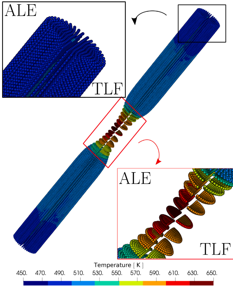
Fig. 22. Rapid stretching of a bar. Comparison of the deformed shapes at time t = 30 \mu\text{s} via M3 model: (Left portion of the bar) the proposed ALE algorithm and (Right portion of the subfigure) Godunov-type Total Lagrangian SPH Framework (TLF) [44]. Colour indicates the temperature profile. A Hencky-based von Mises plasticity model combined with a nonlinear Johnson–Cook hardening rule is used. The parameters related to material properties and ALE motion are detailed in Table 6. (For interpretation of the references to colour in this figure legend, the reader is referred to the web version of this article.)
