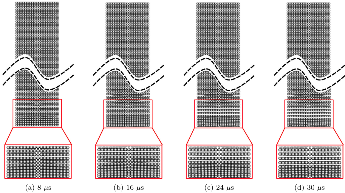
Fig. 20. Rapid stretching of a bar. Two-dimensional view of a series of material mesh deformation at times t = \{8, 16, 24, 30\} \mu s (from left to right). Break lines are used to indicate that a part has been shortened for representation on the figure.
