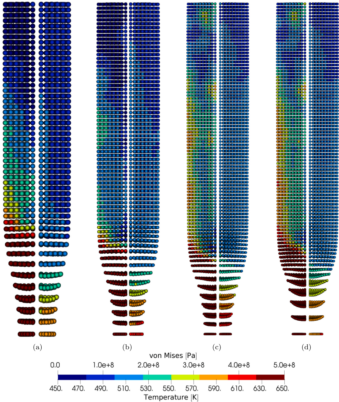
Fig. 21. Rapid stretching of a bar. Comparison of the deformed shapes at time t = 30 \mu\text{s} . The first three columns (left to right) show the refinement of a structure simulated using the proposed ALE algorithm, whereas the last column (at the rightmost position) shows a deformed structure via an alternative Godunov-type Total Lagrangian SPH algorithm [44]. Colour indicates both von Mises (left portion of the subfigure) and temperature (right portion of the subfigure) profiles. A Hencky-based von Mises plasticity model combined with a nonlinear Johnson–Cook hardening rule is used. The parameters related to material properties and ALE motion are detailed in Table 6. (For interpretation of the references to colour in this figure legend, the reader is referred to the web version of this article.)
