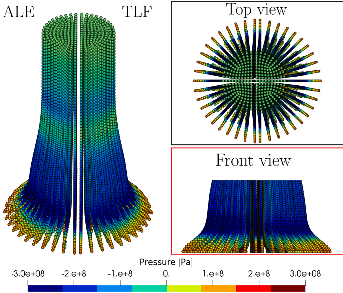
Fig. 17. Taylor bar impact. Comparison of the deformed shapes at time t = 80 \mu\text{s} via M3 model. In each subfigure, left portion of the bar represents the results obtained through the proposed ALE algorithm and the right portion of bar using in-house Total Lagrangian Godunov-type SPH algorithm [44] (TLF). Colour indicates pressure profile. A Hencky-based von Mises plasticity model using linear hardening rule is used (26). The corresponding simulation parameters are summarised in Table 5. (For interpretation of the references to colour in this figure legend, the reader is referred to the web version of this article.)
