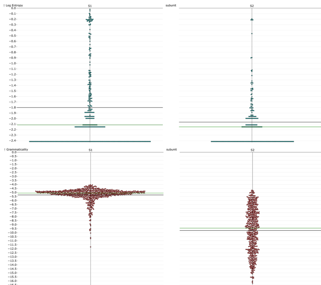
Supplementary Figure 1. Swarm plots for the distributions of entropy and grammaticality for each of the SARS-CoV-2 spike protein subunits S1 and S2. The black line shows the mean while the green line shows the median. For both entropy and grammaticality, the S2 subunit has on average lower scores compared to the S1.
